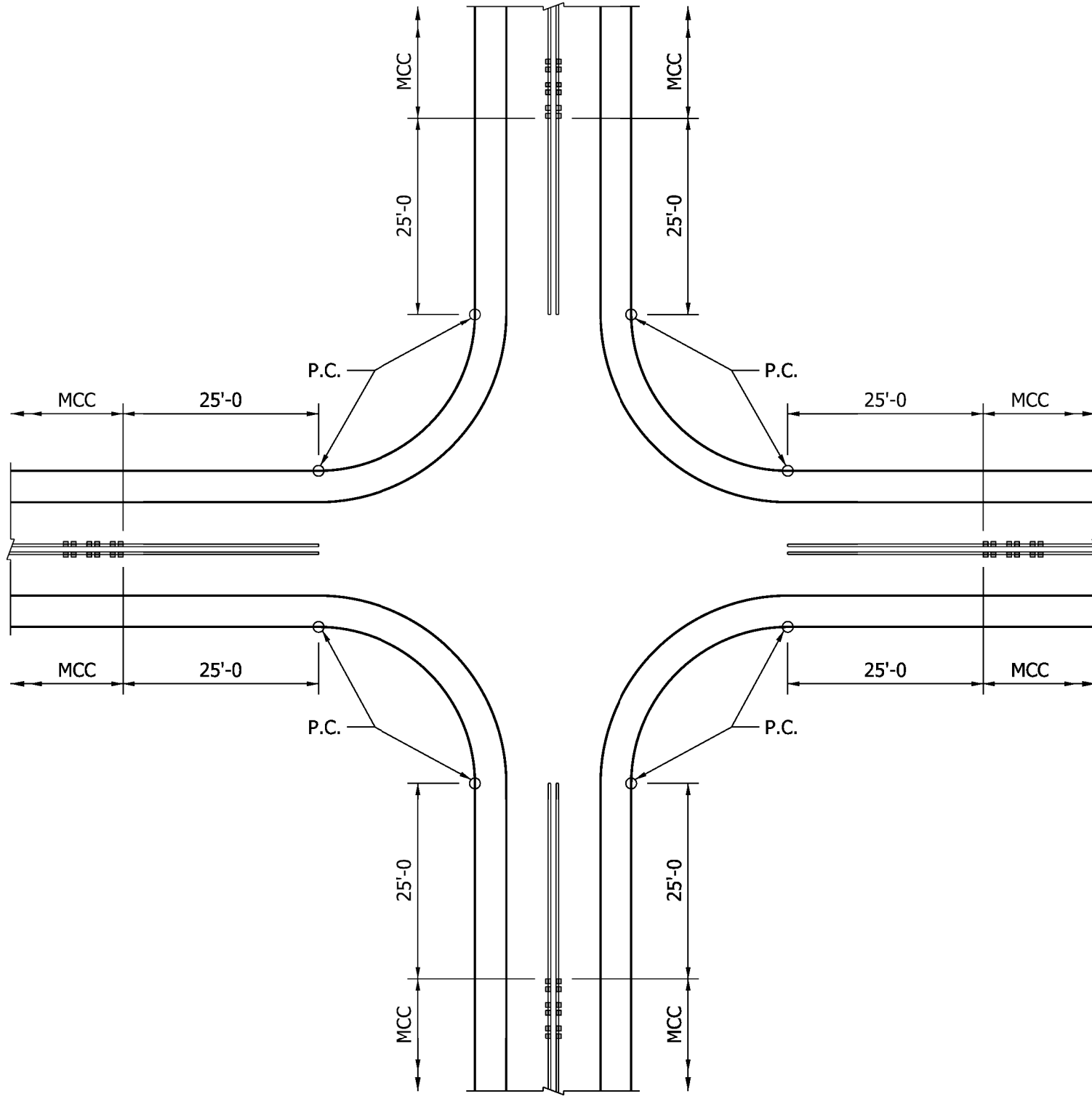
TYPICAL INTERSECTION DETAIL
