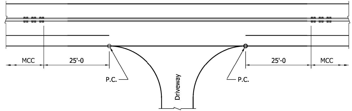
TYPICAL DRIVEWAY DETAIL
